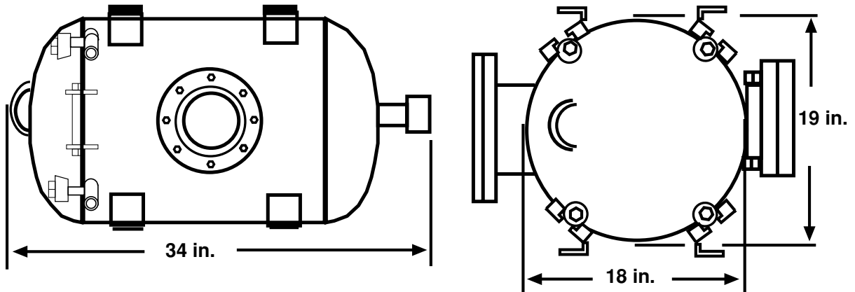
Firing Tank P/N 167-9818
